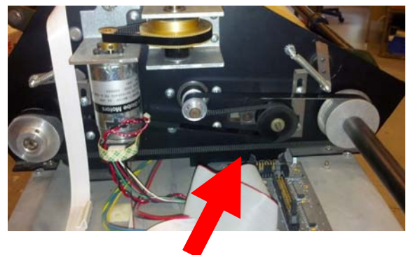
536 Serpentine belt shown above. Part number V40-452-00. NOTE: This part is the same on ALL 536 models
